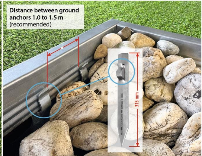
Fixing with ground anchor GEA604315
